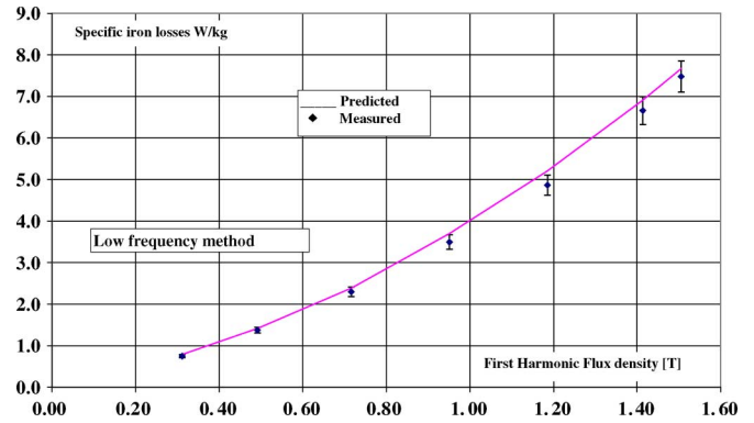
Fig. 7. Measured and predicted specific iron losses using the low-frequency method (fundamental frequency = 50 Hz and percentage error bars = \pm 5\% ).
