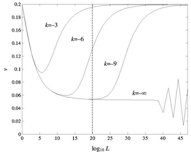
FIG. 5. Effective Poisson's ratio of a Sierpinski carpet vs dimensionless size L for different negative values of k .
