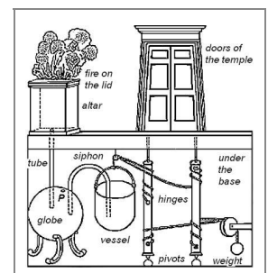
Figure 3. When the fire on the altar has grown hot, the pressure in the globe increases, driving out some liquid contained there through the siphon into a suspended vessel. The vessel, descending under the weight, will tighten the chains and open the doors. When the fire is extinguished, the pressure decreases, the water flows back into the globe through the bent siphon from the suspended vessel. The weight suspended will preponderate and shut the doors.
