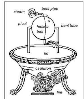
Figure 1 Aeolipile or the Hero's Machine. Heating the water in the cauldron with a fire, the steam enters the hollow ball through the bent tube and passes out through the two bent pipes, causing the ball to revolve.
