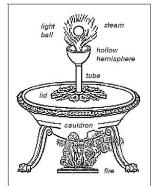
Figure 2. The ball is floating suspended by the Bernoulli Effect in the flowing steam
