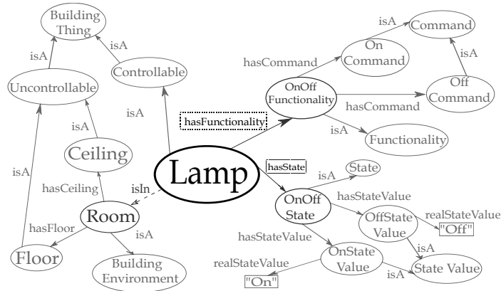
Fig. 1. Ontology fragment showing a DogOnt Lamp class.
