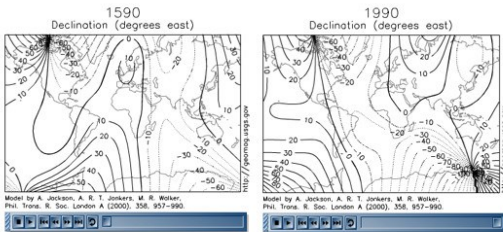
Figure 9: Thanks to the works of the USGS Geomagnetism Program [18], we have the possibility to see the evolution of the magnetic declination. Here we reproduce two frames of a movie, concerning the period from 1590 to 1990, made according to data in Ref.19.
