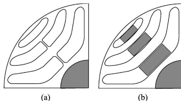
Fig. 1. Schematic of (a) TLSyR rotor and (b) PMASR rotor.
