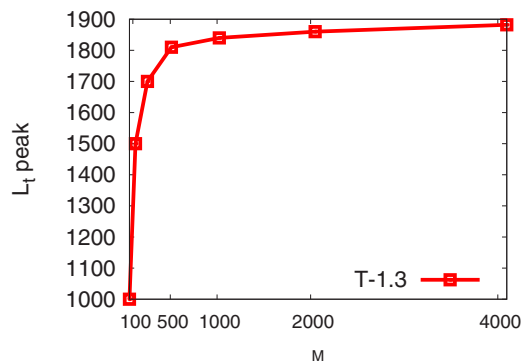
FIG. 7. Number of most likely decimated couplings, estimated by the maximum point of \mathcal{L}_t , as a function of the number of samples M . We can clearly see that the maximum point of \mathcal{L}_t tends toward x^* = 1888 , which is the correct expected number of zero couplings in the system.
